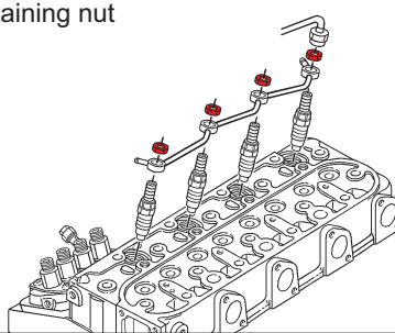
Overflow pipe assembly retaining nut
