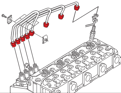
Injection pipe retaining nut
