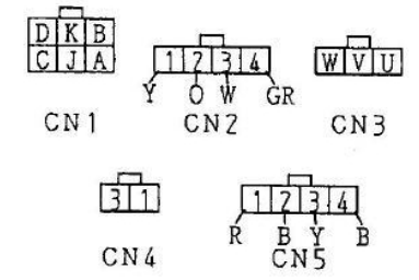
CONNECTOR ARRANGEMENT (WIRING VIEW)
