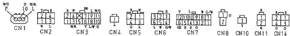
CONNECTOR (VIEW FROM WIRING SIDE)
