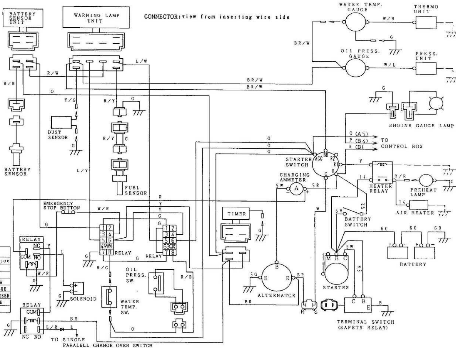
49WX 63QX RELAY INSIDE CONNECTION
