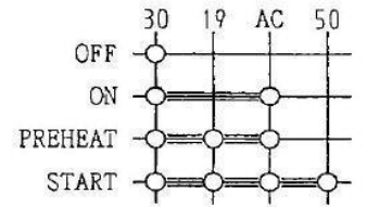
STARTER SWITCH CONNECTION
