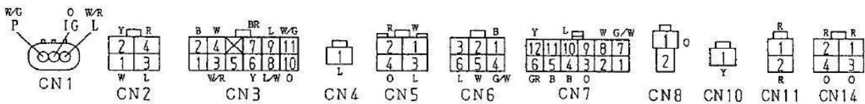
CONNECTOR (VIEW FROM WIRING SIDE)
