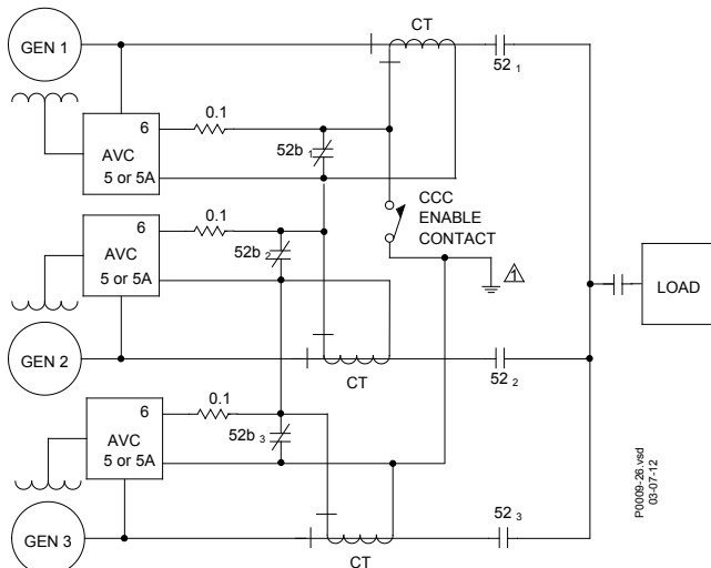
Figure 8. Cross-Current Compensation
